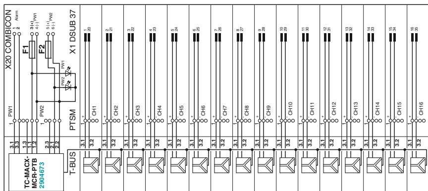
Схема соединений TC-D37SUB-ADIO16-EX-P-UNI и TC-D37SUB-AIO16-EX-PS-UNI
